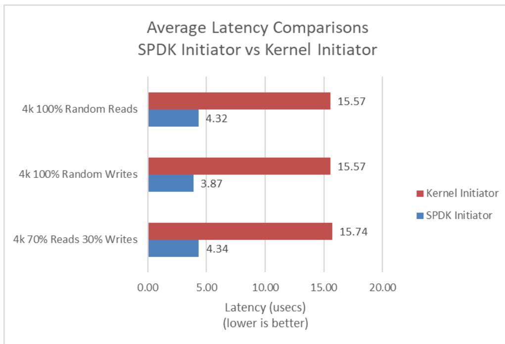
Figure 9: Average I/O Latency Comparisons at QD=1 between SPDK and Linux Kernel NVMe-oF RDMA Initiator for various workloads against SPDK NVMe-OF Target
