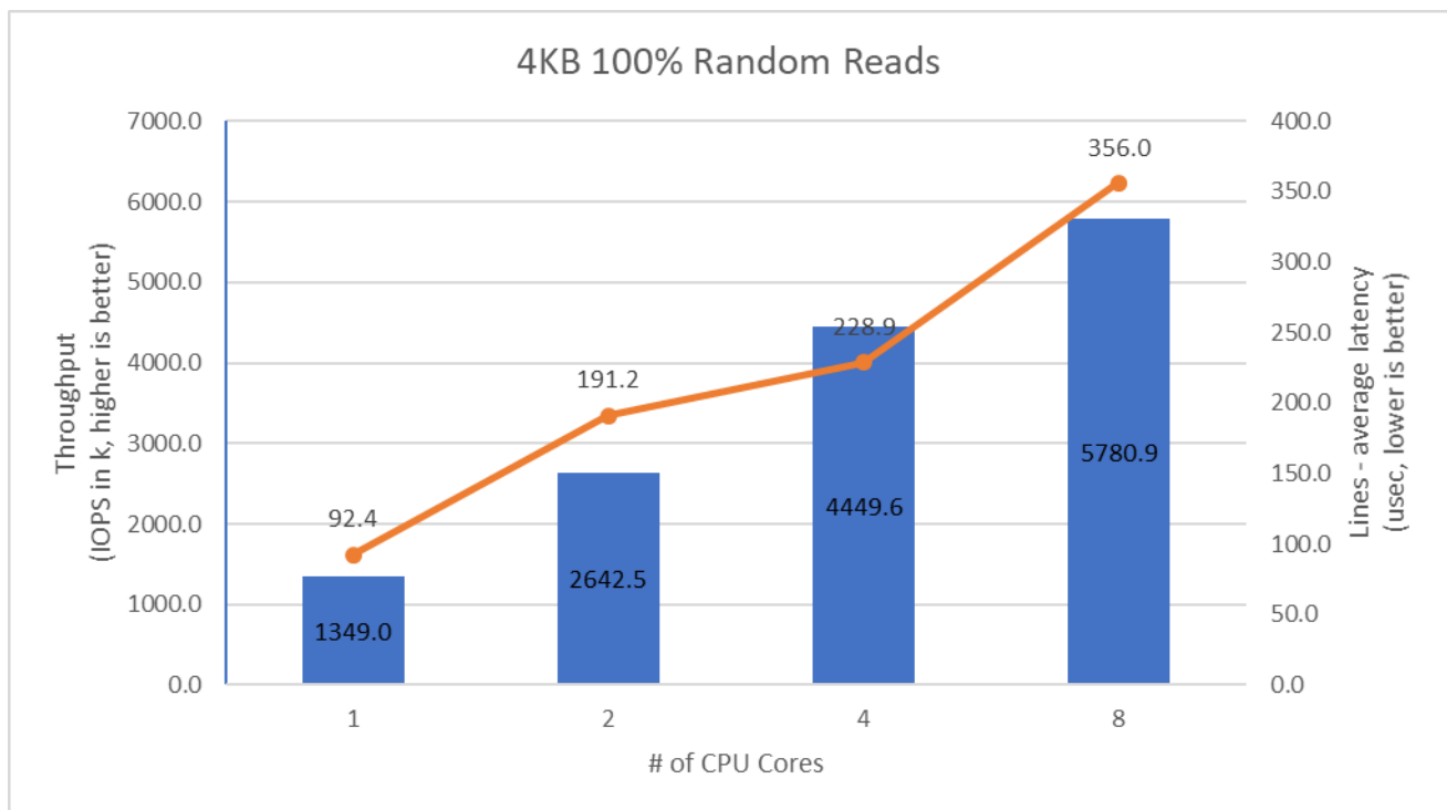
Figure 5: SPDK NVMe-oF RDMA Initiator I/O core scaling: IOPS vs. Latency while running 4KB 100% Random Read workload at QD=128
