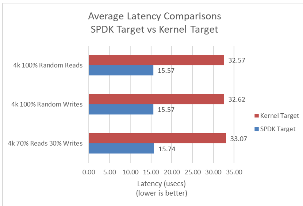
Figure 8: Average I/O Latency comparisons at QD=1 between SPDK and Linux Kernel NVMe-oF RDMA Target for various workloads using the Linux Kernel Initiator
