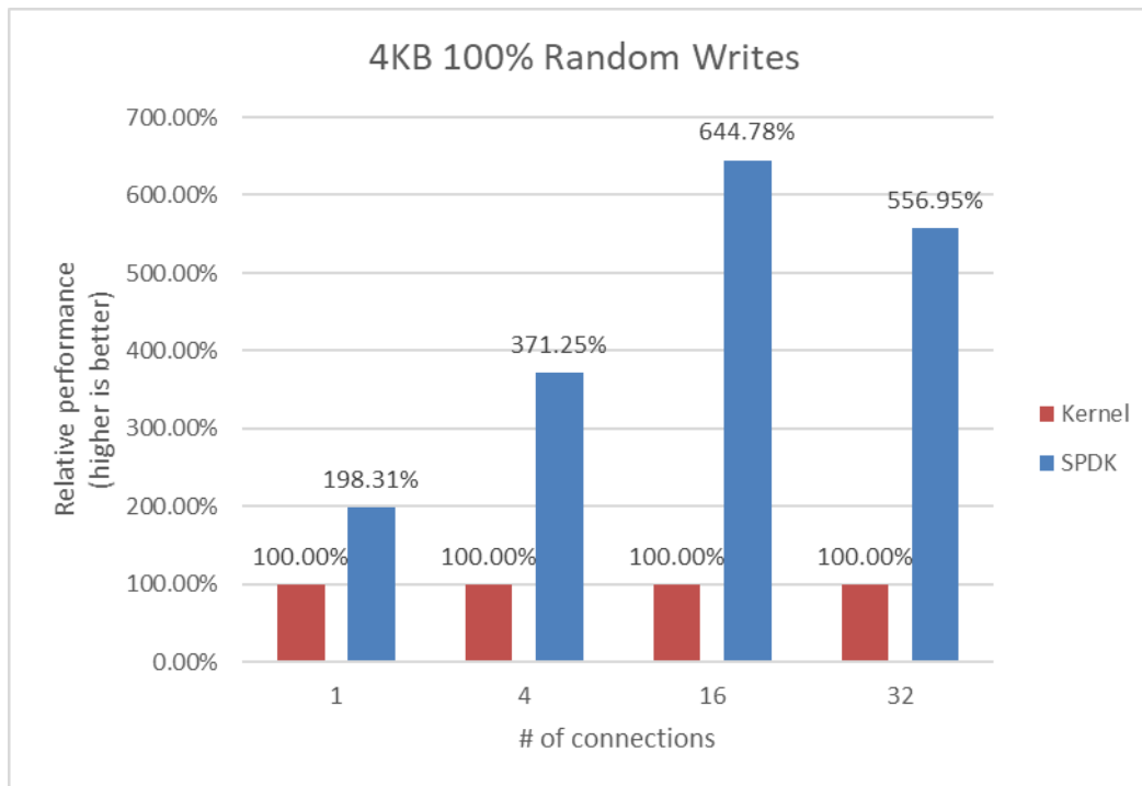
Figure 11: Relative Performance Comparison of Linux Kernel vs. SPDK NVMe-oF RDMA Target for 4KB 100% Random Write QD=32, using Kernel Initiators
