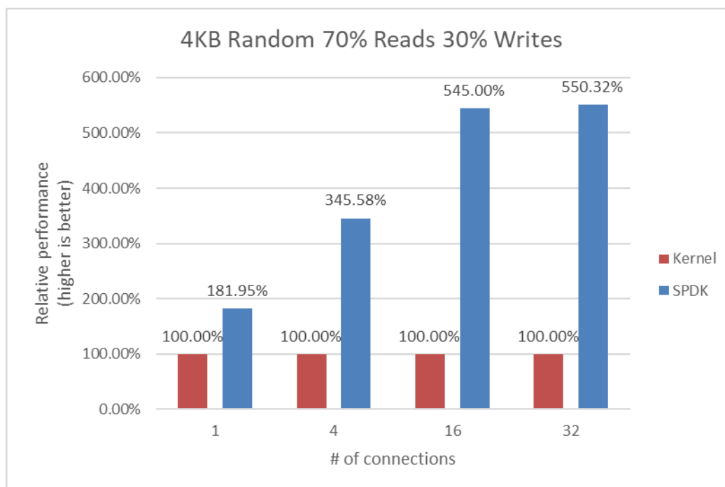
Figure 12: Relative Performance Comparison of Linux Kernel vs. SPDK NVMe-oF RDMA Target for 4KB Random 70% Read 30% Write QD=32, using Kernel Initiators
