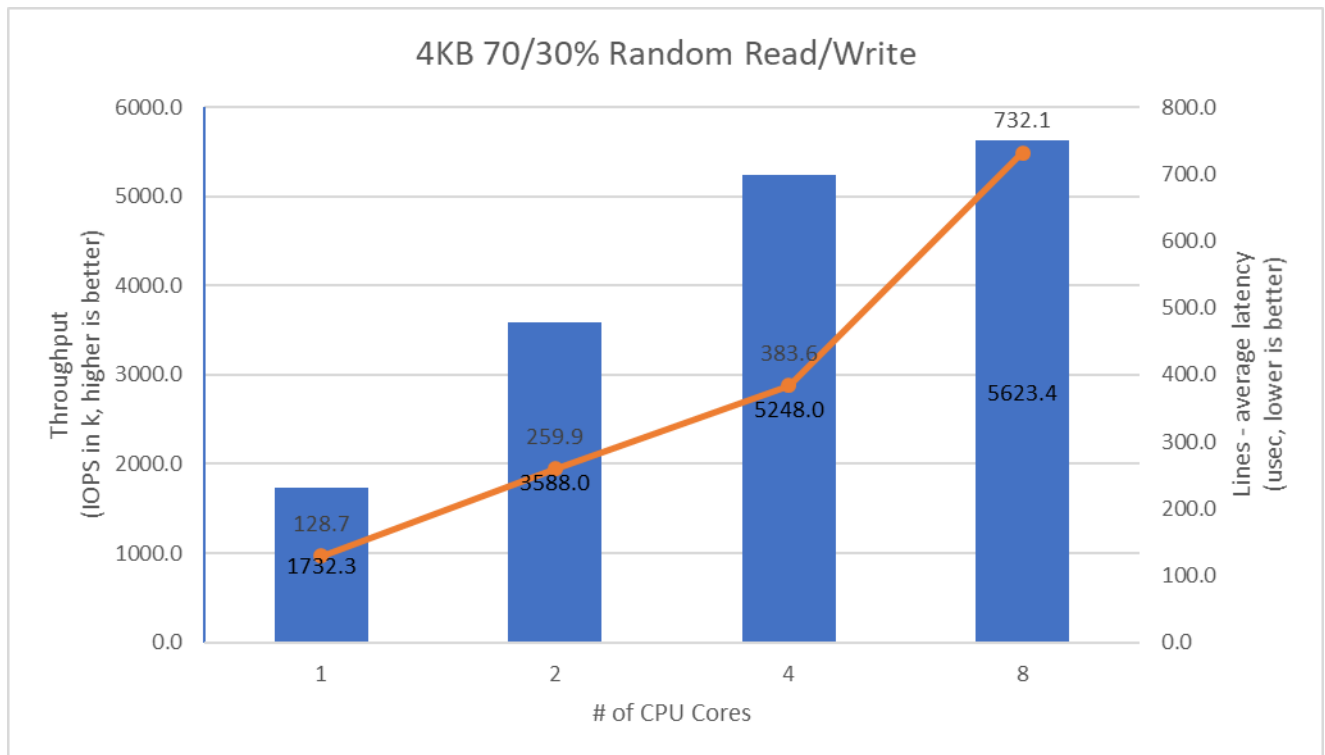
Figure 7: SPDK NVMe-oF RDMA Initiator I/O core scaling: IOPS vs. Latency while running 4KB Random 70% Read 30% Write workload at QD=256
