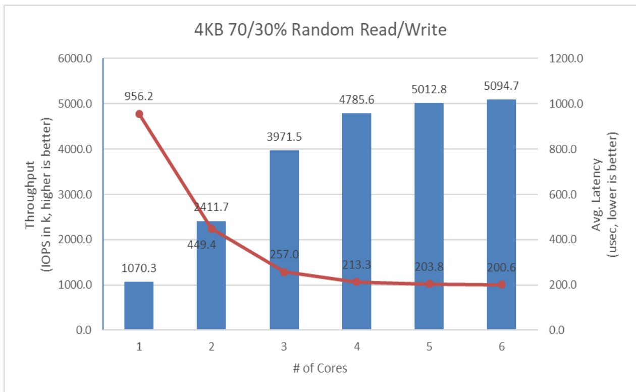
Figure 4: SPDK NVMe-oF RDMA Target I/O core scaling: IOPS vs. Latency while running 4KB Random 70% Read 30% Write workload at QD=64
