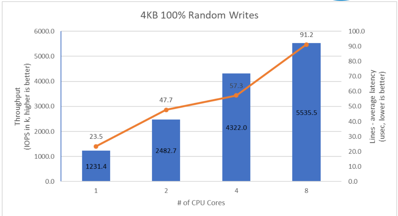
Figure 6: SPDK NVMe-oF RDMA Initiator I/O core scaling: IOPS vs. Latency while running 4KB 100% Random Write workload at QD=32
