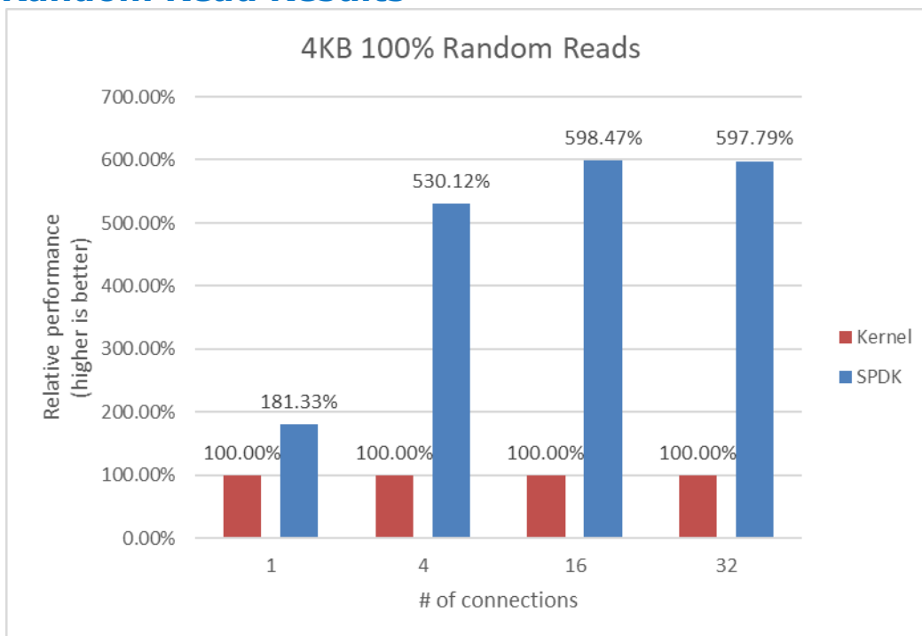
Figure 10: Relative Performance Comparison of Linux Kernel vs. SPDK NVMe-oF RDMA Target for 4KB 100% Random Read QD=32, using Kernel Initiators
