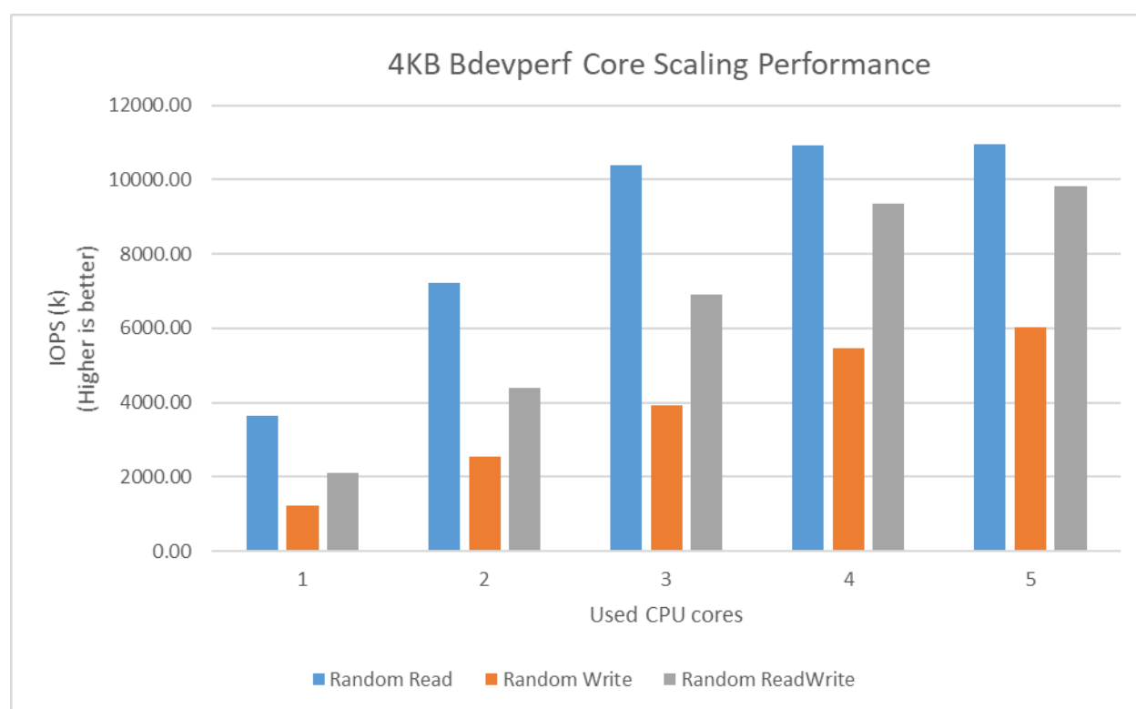
Figure 6: SPDK NVMe BDEV I/O Cores Scalability with addition of SSDs (4KB 100% Random Read IOPS at QD=128; 4KB 100% Random Write IOPS at QD=32; 4KB 70/30 Random Read/Write IOPS at QD=128)
