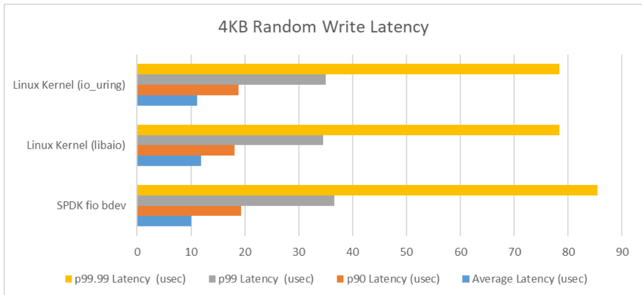
Figure 10: SPDK bdev vs Linux Kernel Latency comparison (4KB Random Write)
