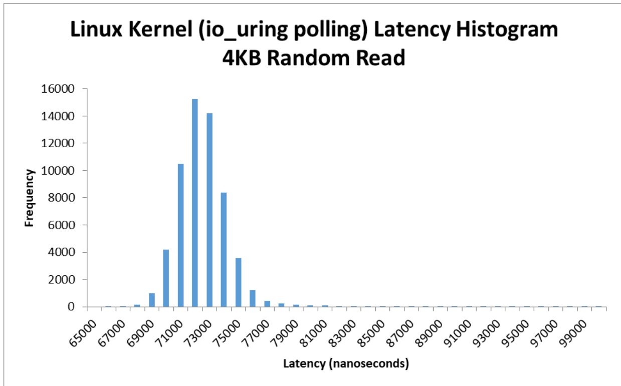
Figure 13: Linux Kernel (io_uring polling) 4KB Random Read Average Latency Histogram (QD=1, Runtime=900s, fio, sampling interval = 15msec)
